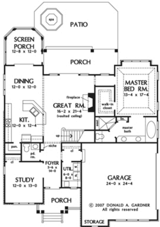
FIRST FLOOR PLAN PLAN NO. 1216
