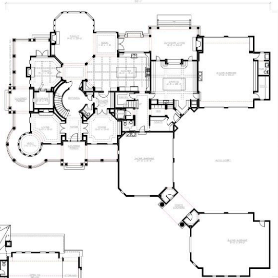
MAIN FLOOR
