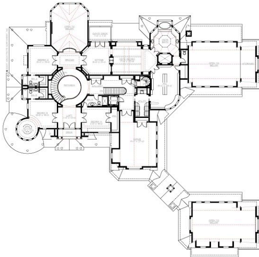
UPPER FLOOR
